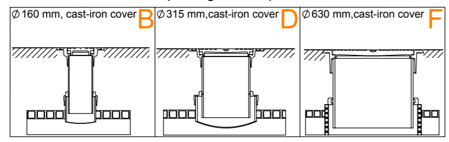
Service openings for asphalt area
